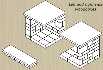
Compact Hearth 40" W x 12" D x 6" H
