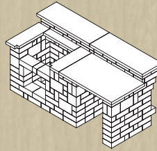
Grand Island Bar/Grill with Refrigerator Opening 96" W x 48" D x 46" H
