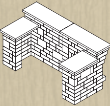
Grill Surround 96" W x 48" D x 46" H
