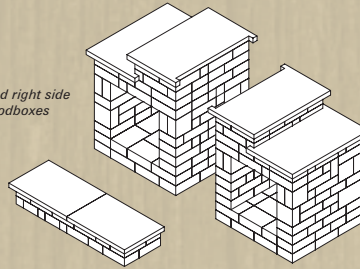
Grand Hearth 60" W x 20" D x 10" H
